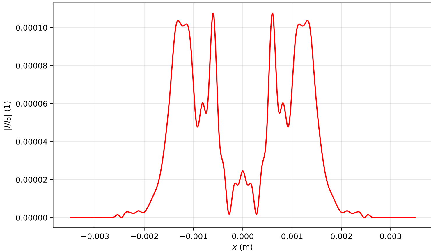
Intensity profile I(x, y = 0, z = 2.946)/I_0 , P_{in}=8.0P_{cr} , artificial time
